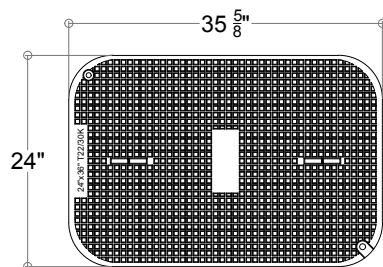
COVER TOP VIEW
