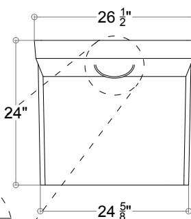
BOX SIDE VIEW
